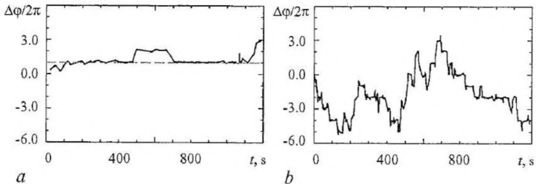
Fig. 12. Phase differences for the fast synchronous (a) and for the fast non-synchronous dynamics (b). The given examples are obtained for the time series of hypertensive rats shown in Fig. 7, c and b, respectively
